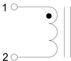
SCHEMATIC DRAWING
